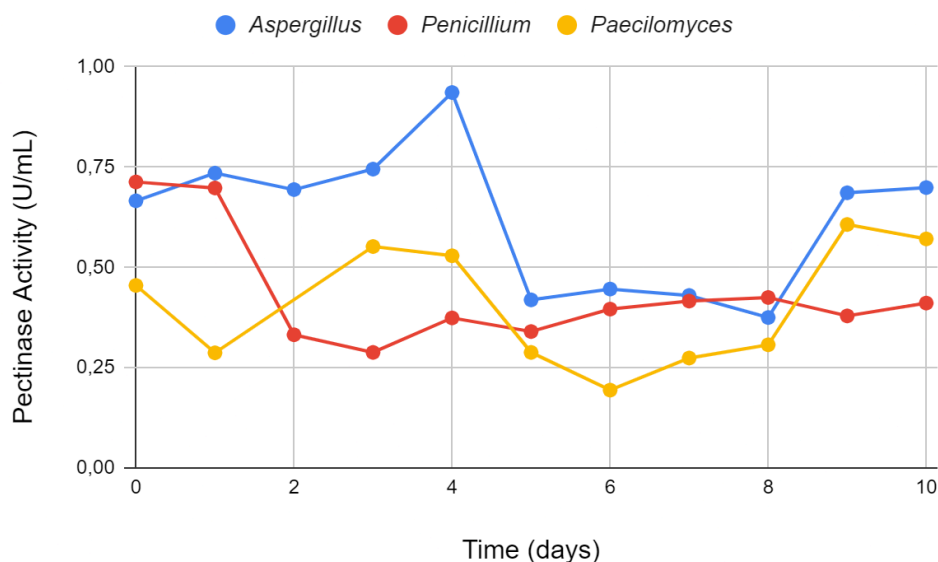
Figure 1. Pectinase production comparison in assays with Penicillium sp., Paecilomyces sp. TP08 and Aspergillus sp. NA01
